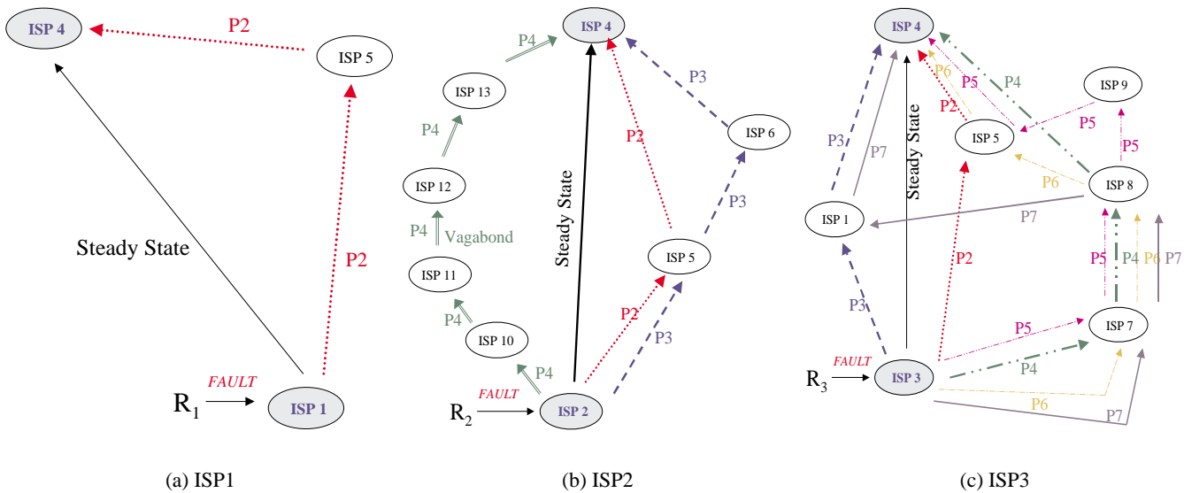
Fig. 3. Example of backup paths explored during process of repair for routes from a Japanese provider to three different ISP routers at the California Mae-West exchange point.
